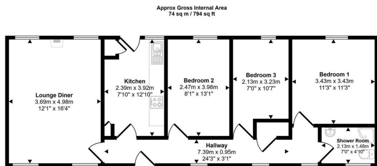
Floorplan
